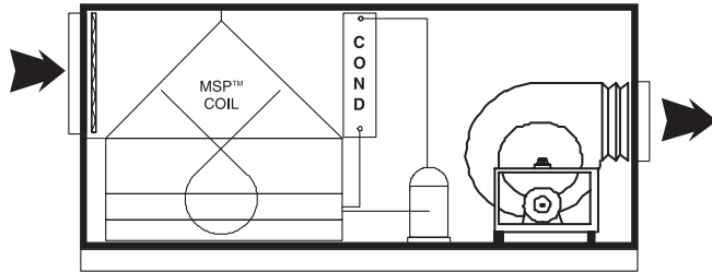
DH Integral (Indoor/Outdoor)
