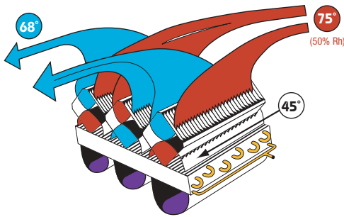
DHOP Series, 3,000-CFM Indoor Air Dehumidifier; Clean Room, Portland, OR—Features Super-Efficient MSP™ Technology
